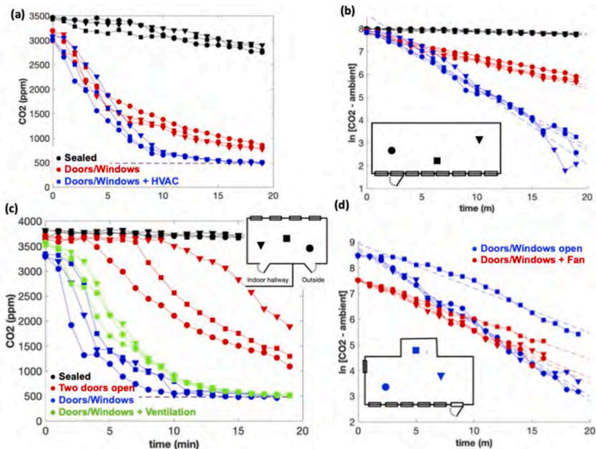
Fig. 6. (a) \text{CO}_2 decay measured in three different locations of a Coastal California classroom, under three conditions: closed doors and windows (black), open doors and windows (red) and open doors and windows plus HVAC (blue). The dashed line indicates ambient \text{CO}_2 level, measured separately. (b) Log-linear plot of data from panel (a); ACH determined from slopes obtained from linear regression fits (dashed). No difference appears between different locations within the room. (c) Room with non-exponential decay and positional lag. (d) Classroom with an ‘alcove’. (For interpretation of the references to color in this figure legend, the reader is referred to the Web version of this article.)
